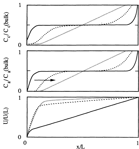
FIG. 2. The concentration of cations and of anions that would be found at different stages of growth of a smooth deposit on the cathode (solid line: t = 10^2 s; dashed line: 10^3 s; dotted line: 10^4 s), and the potential difference (bottom). As one notices, the potential near the cathode increases progressively. A large field appears near the cathode. An excess of positive charges forms in a thin layer near the cathode, which is responsible for the curvature of the potential. The bulk of the solution is quasineutral. Here, due to unrealistically small concentrations ( C = 10^{11} \text{ cm}^{-3} ), the charged layer appears thick. In usual conditions, its thickness is very small, of the order of a few micrometers.
