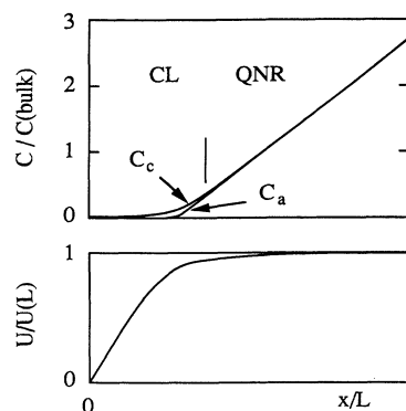
FIG. 3. The potential and the concentration through the cell, in the case of smooth deposition, when the steady state is achieved. Unrealistically small values of the concentration are used ( C = 10^{10} \text{ cm}^{-3} ), so that the two zones can be clearly distinguished. There is a charged layer (CL) near the cathode, where an excess of cations and a large field are found. The rest of the cell is quasineutral (QNR), but there remains a very small excess of positive charges.
